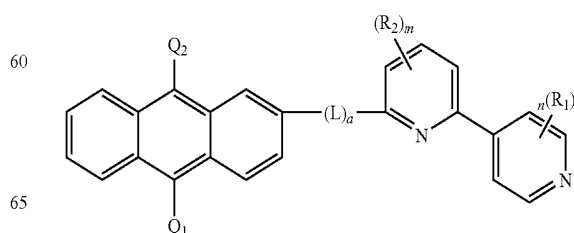
Formula 3a
