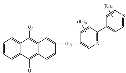
Formula 3b
