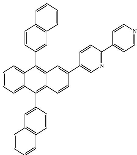
Compound 15
