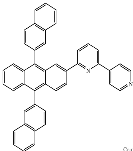
Compound 2
