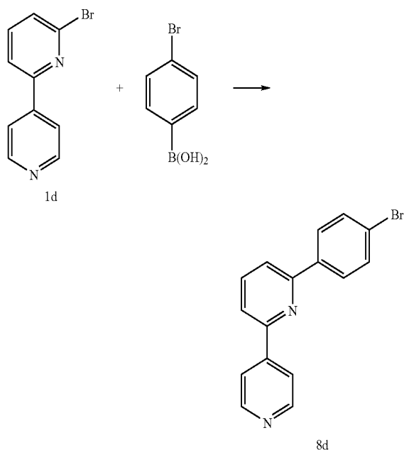
Reaction Scheme 3
