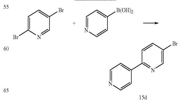
Reaction Scheme 6
