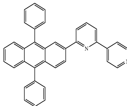
Compound 4
