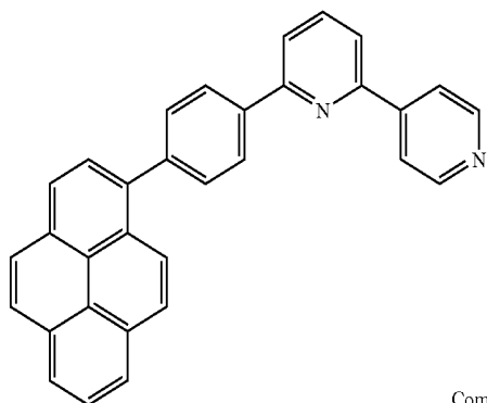
Compound 3
