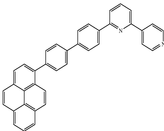
Compound 3
