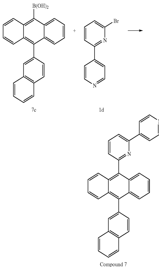
Reaction Scheme 2
