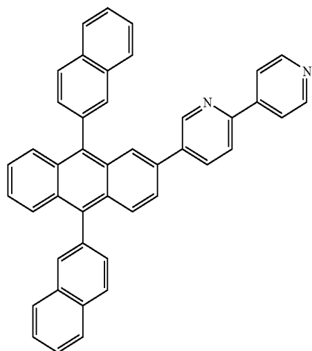
Compound 15
