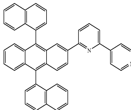
Compound 5
