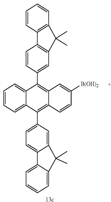
Reaction Scheme 5
