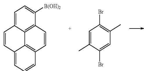
Reaction Scheme 8
