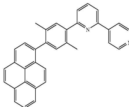
Compound 27
