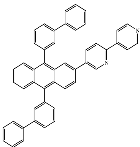
Compound 14
