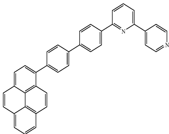
Compound 4
