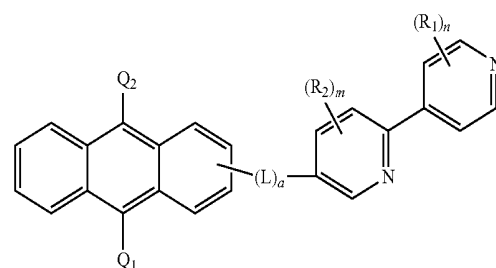
Formula 2c
