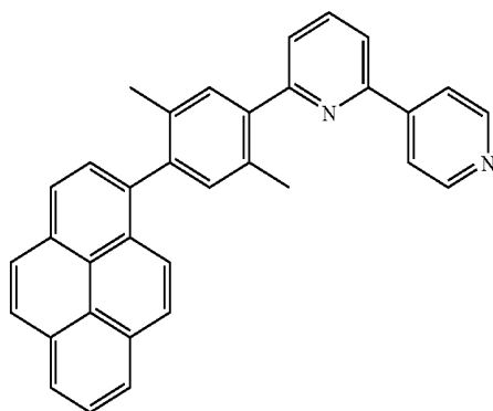
Compound 27
