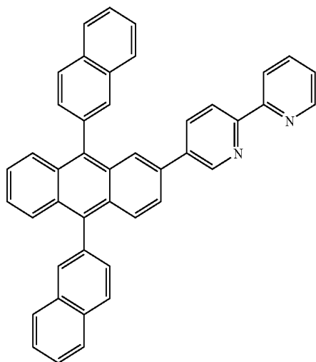
Compound E
