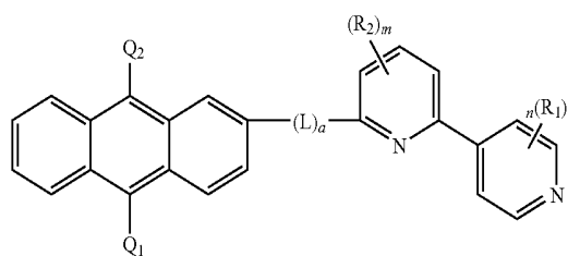
Formula 3b
