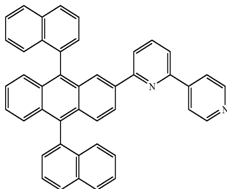
Compound 5
