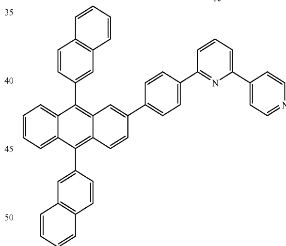
Compound 25
