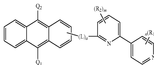
Formula 2b
