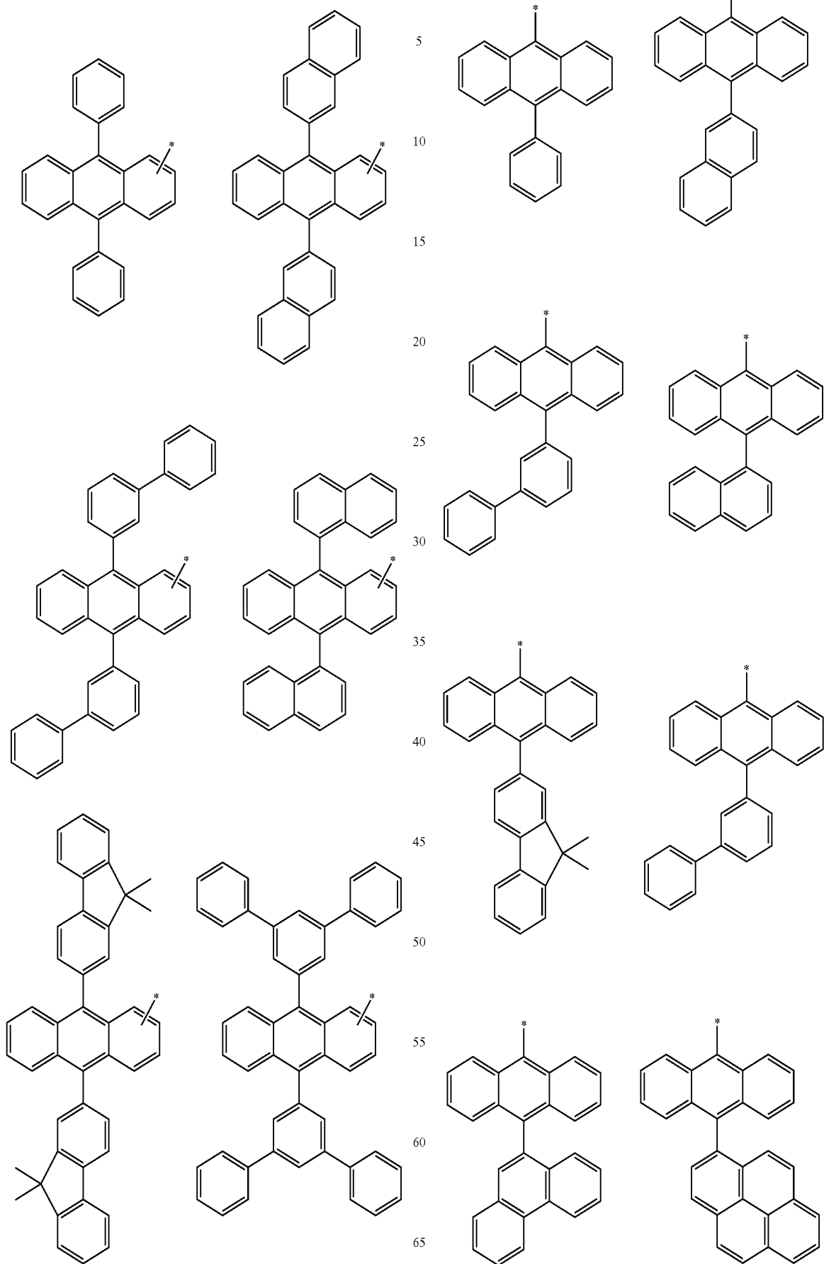
Formula 4
