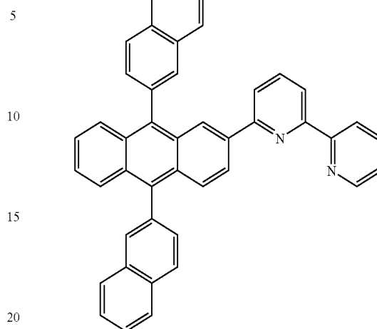
Compound C
