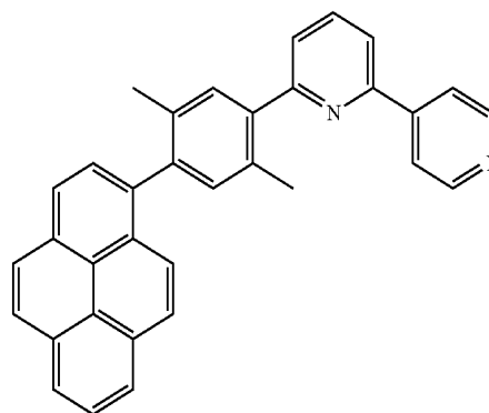
Compound 27
