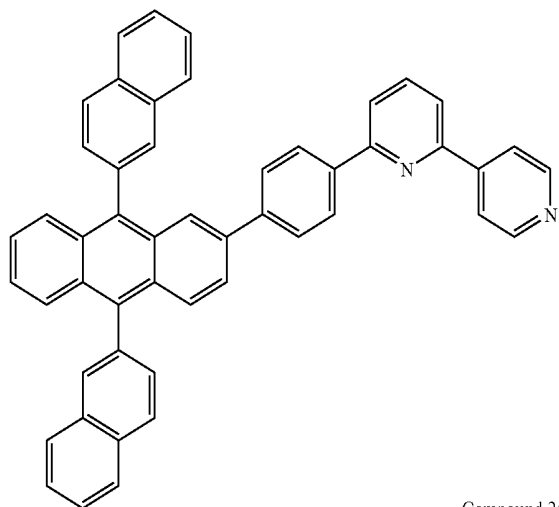
Compound 26
