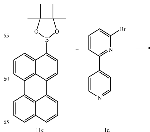
Reaction Scheme 4
