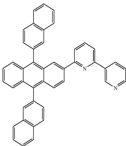
Compound B
