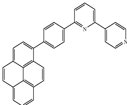
Compound 2
