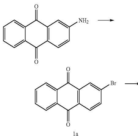
Reaction Scheme 1
