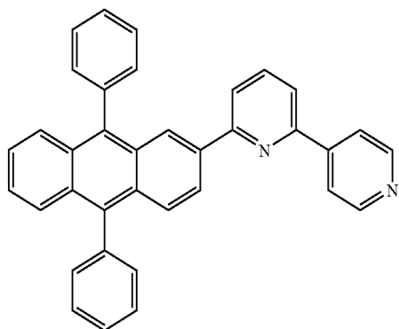
Compound 4
